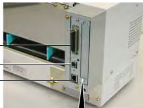
Parallel Connector
